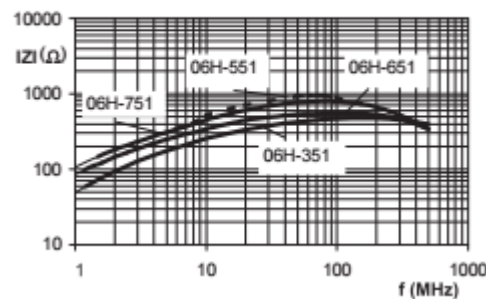
Typical |Z| vs Frequency (f)
