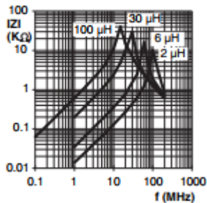
Typical |Z| vs Frequency(f)
