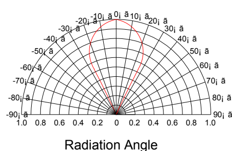
Radiation Characteristics
