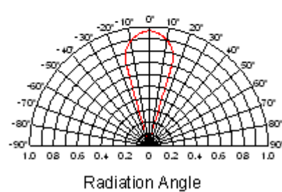
Radiation Characteristics
