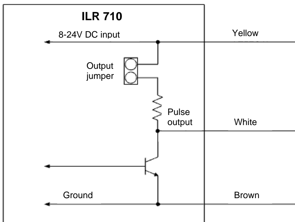
Figure 13: ILR 710 wiring
