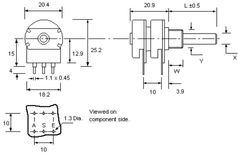
SPINDLE END VIEW
