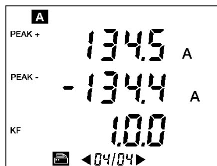
Figure 63: The printer icon flashes during the transfer of the information to the thermic serial printer.
