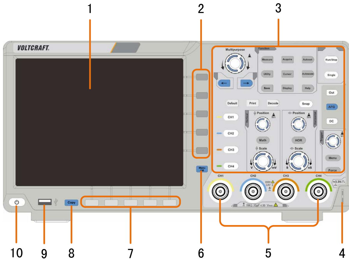
Figure 3-1 Front panel
