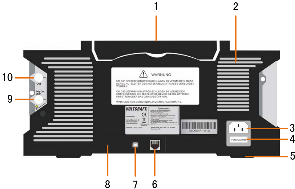
Figure 3-2 Rear Panel
