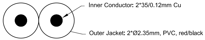
Cable Structure
