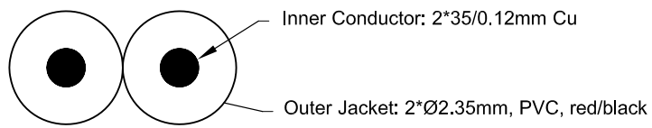
Cable Structure
