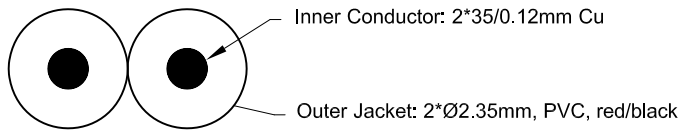
Cable Structure
