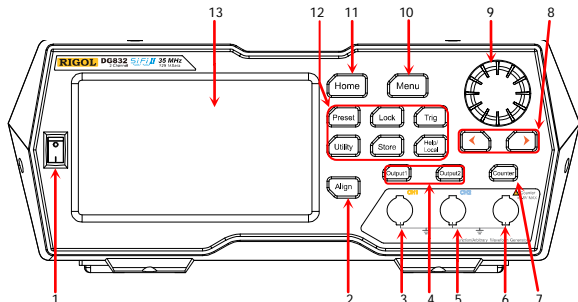
Figure 1 Front Panel
