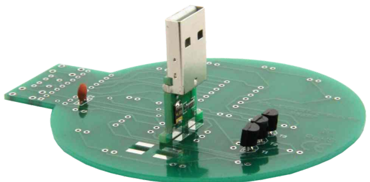
USB connector position for vertical USB port:
