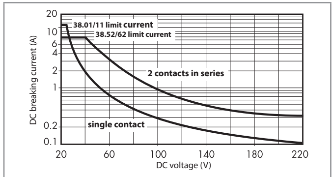
H 38 - Maximum DC1 breaking capacity, 1 Pole 16 A and 2 Pole 8 A
