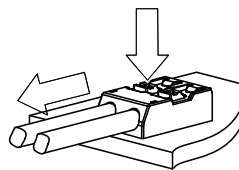
Fig. 5.3 Disconnecting the wire
