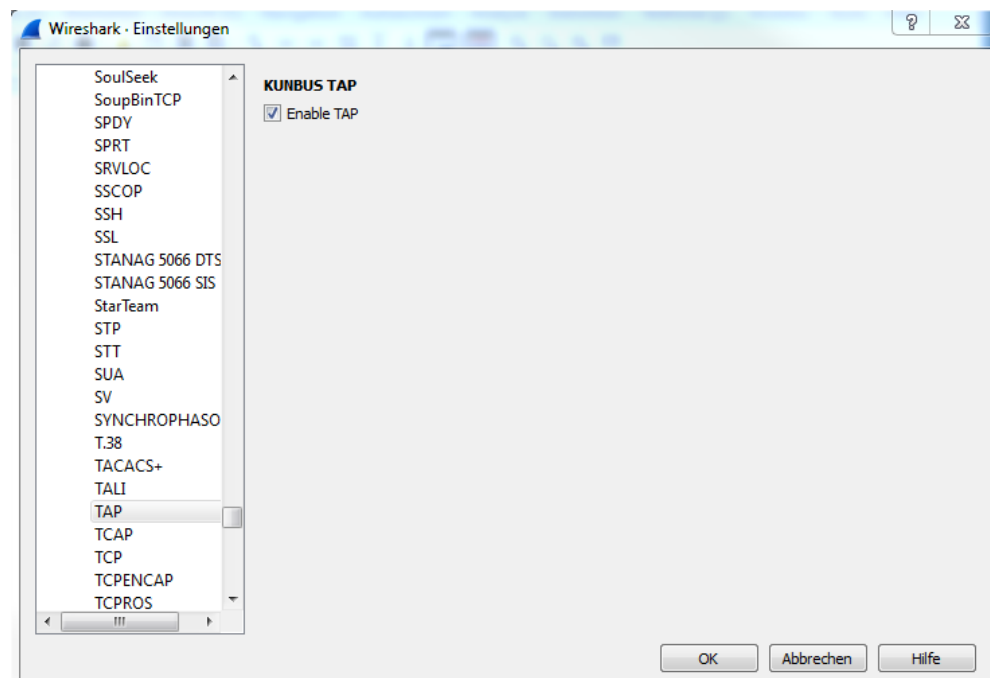
Illustration 6: Wireshark plugin
