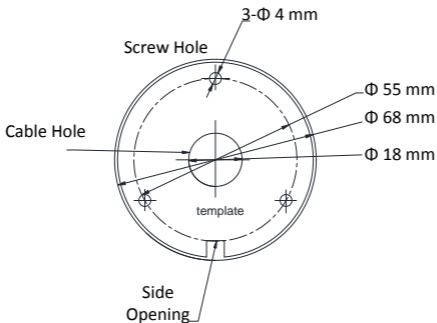
Figure 2-1 The Drill Template
