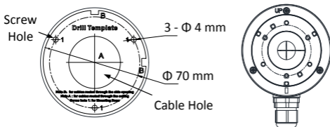
Figure 2-4 The Drill Template
