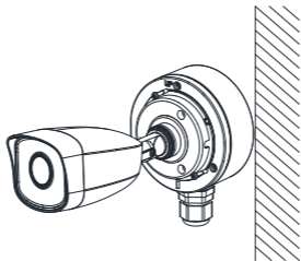
Figure 2-7 Combine Junction Box's Cover with its Body
