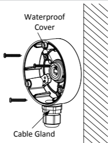
Figure 2-6 Fix the Junction Box on the Wall
