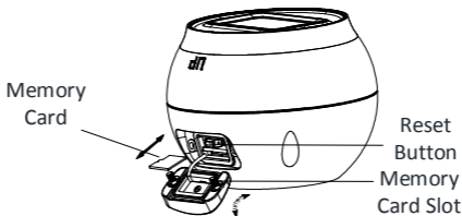
Figure 2-2 Install the Memory Card
