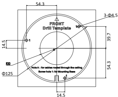
Figure 2-4 The Drill Template
