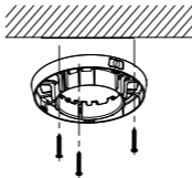
Figure 2-5 Fix the Mounting Base
