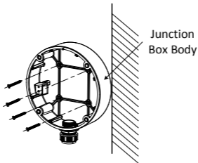
Figure 2-14 Secure the Junction Box's Body on the Wall
