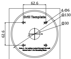
Figure 2-12 Drill Template
