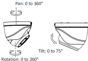
Figure 2-7 Adjust Surveillance Angle
