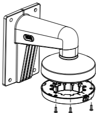
Figure 2-10 Install the Mounting Base to the Bracket
