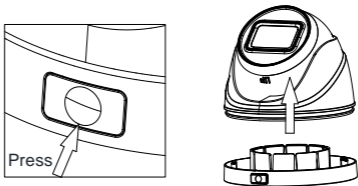
Figure 2-3 Disassemble the Camera
