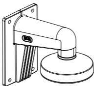
Figure 2-9 Install the Bracket
