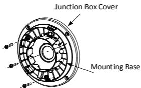
Figure 2-13 Fix Mounting Base on the junction box's Cover
