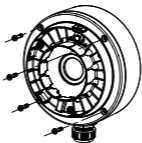
Figure 2-15 Combine the Junction Box's Cover with its body
