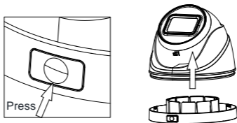
Figure 2-16 Disassemble the Camera
