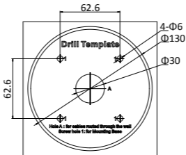
Figure 2-17 Drill Template
