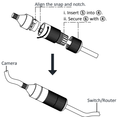
Figure 2-22 Waterproof Accessory Installation
