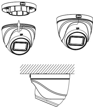
Figure 2-6 Install the Camera Body
