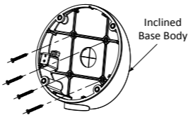
Figure 2-19 Fix the Inclined Base's boy on Ceiling/Wall
