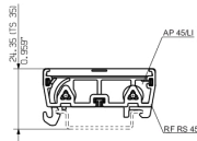
RAIL MOUNTING
