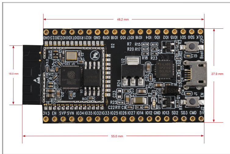
Figure 1-1. ESP32-DevKitC Dimensions
