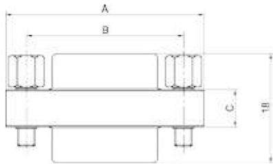
Gender Changer
