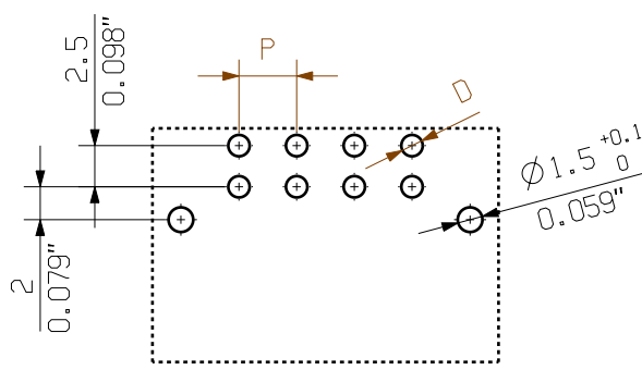
HOLE PATTERN
