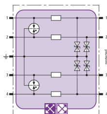
Basic circuit diagram BXT ML4 BE 48
