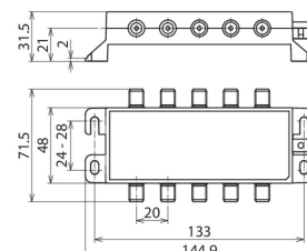
Dimension drawing DGA FF5 TV
