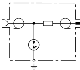
Basic circuit diagram DGA GF TV
