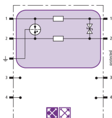
Basic circuit diagram BXT ML2 BD 180
