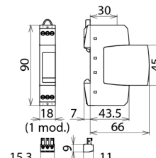
Dimension drawing DR M 2P 30 FM
