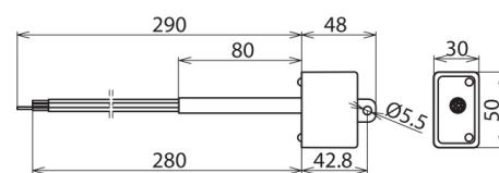
Dimension drawing DCOR L 2P 275 SO IP
