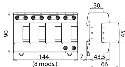
Dimension drawing DV M TT 255
