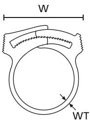
SNP - Snapper Hose Clip (front view)
