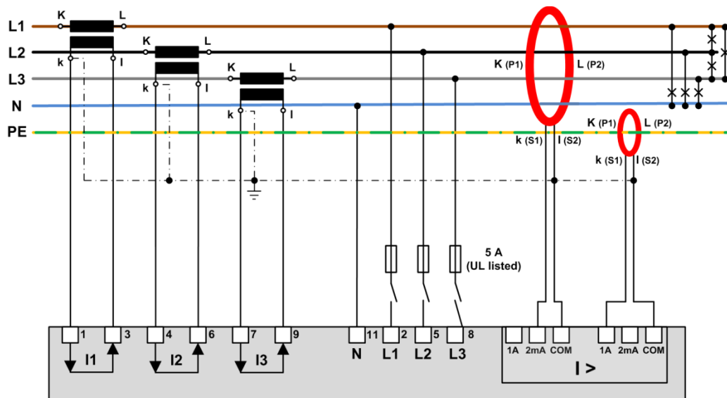
Example: Fault current monitoring in a TNS system
