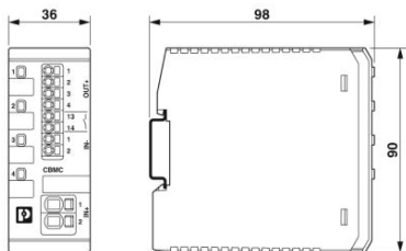
Product drawing
