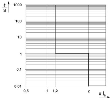
Trigger characteristic in the DC range
