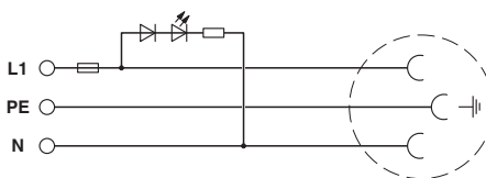
Circuit diagram
