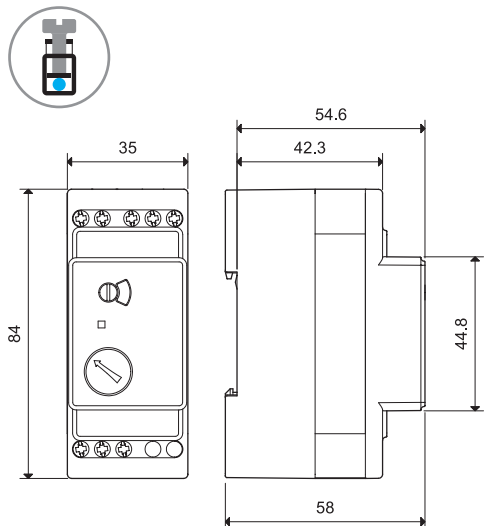
72.01/11 Screw terminal
