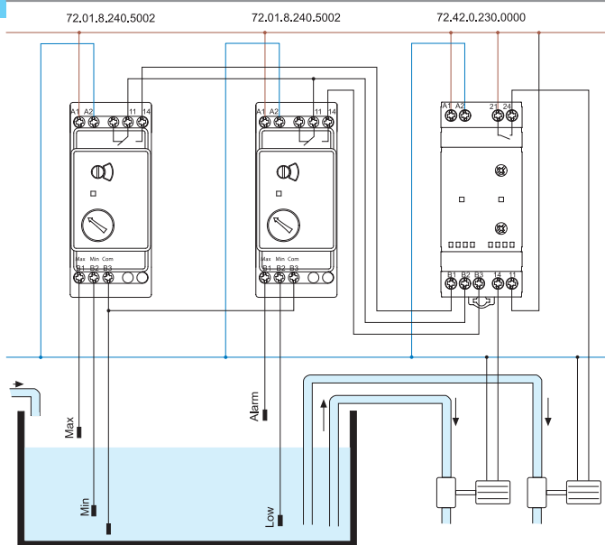
72.01/11 Screw terminal
