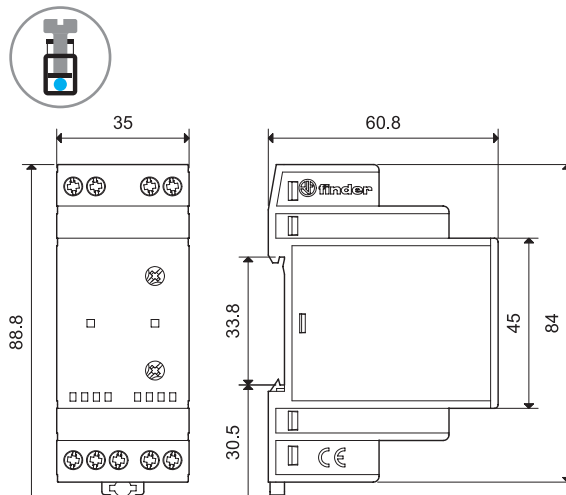
72.42 Screw terminal
