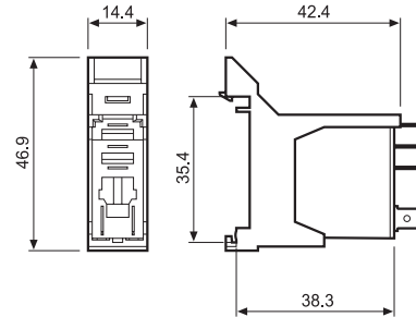
046.07 with relay
