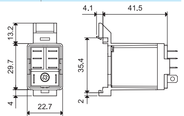
056.27 with relay
