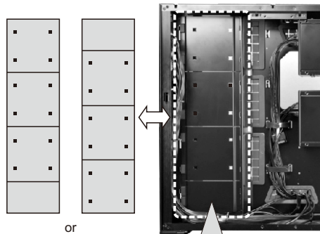
Press to release the HDD tray
