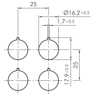
Drilling pattern:
