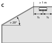
Alternative positioning of the smoke alarm
