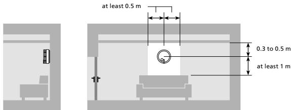
Smoke alarm wall installation
