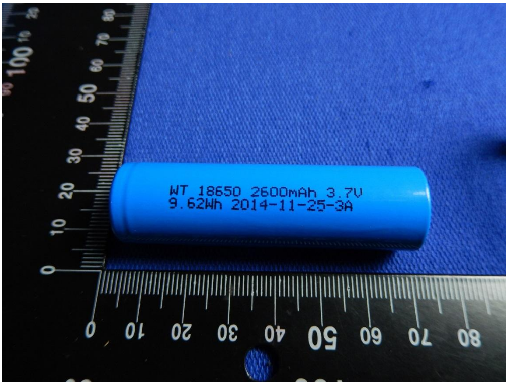
Battery (WT18650 3,7V 2600mAh 9,62Wh)
