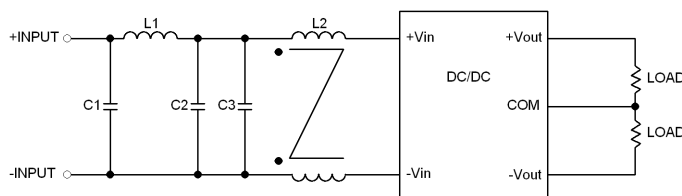
Dual Output
