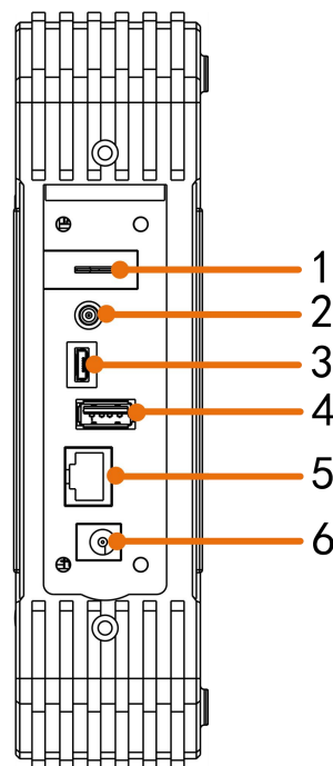
Figure 3-2 Rear Panel
