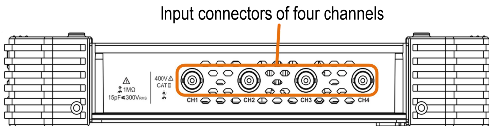
Figure 3-3 Top Panel Overview
