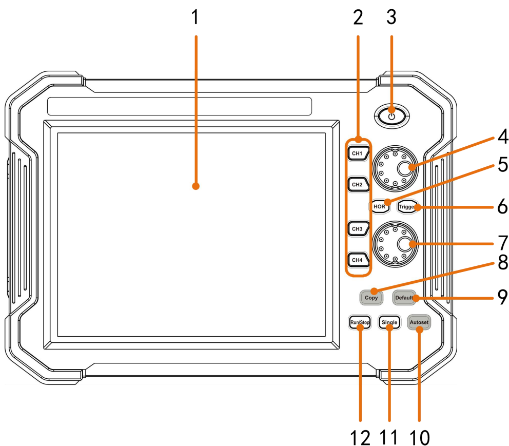
Figure 3- 1 Front panel
