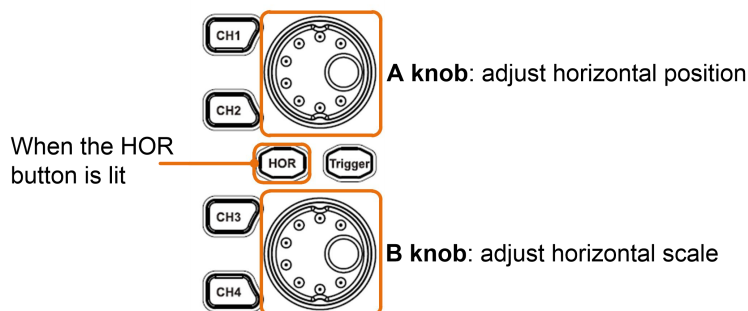
Figure 3- 11 Horizontal Control
