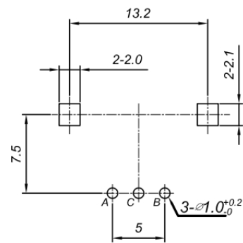
Mounting hole detail
