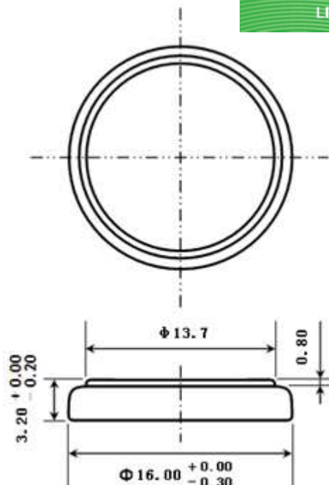
Dimension Drawing
