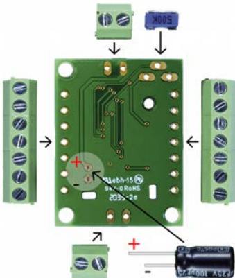
Assembly
