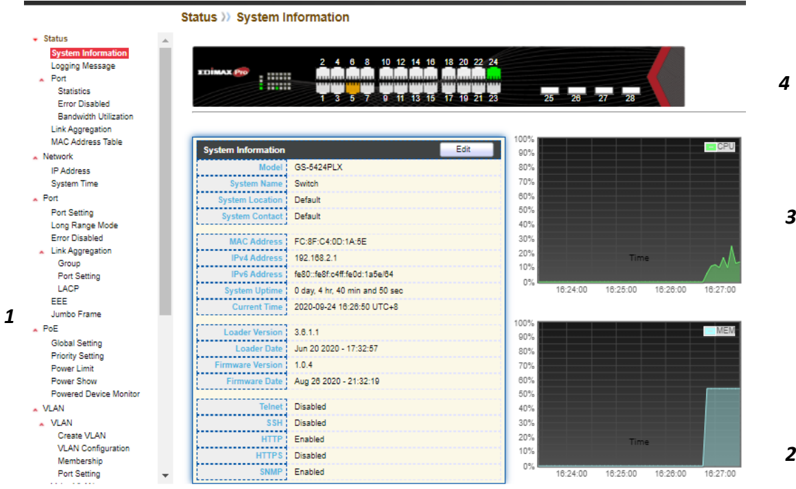
Figure 11 - User Interface
