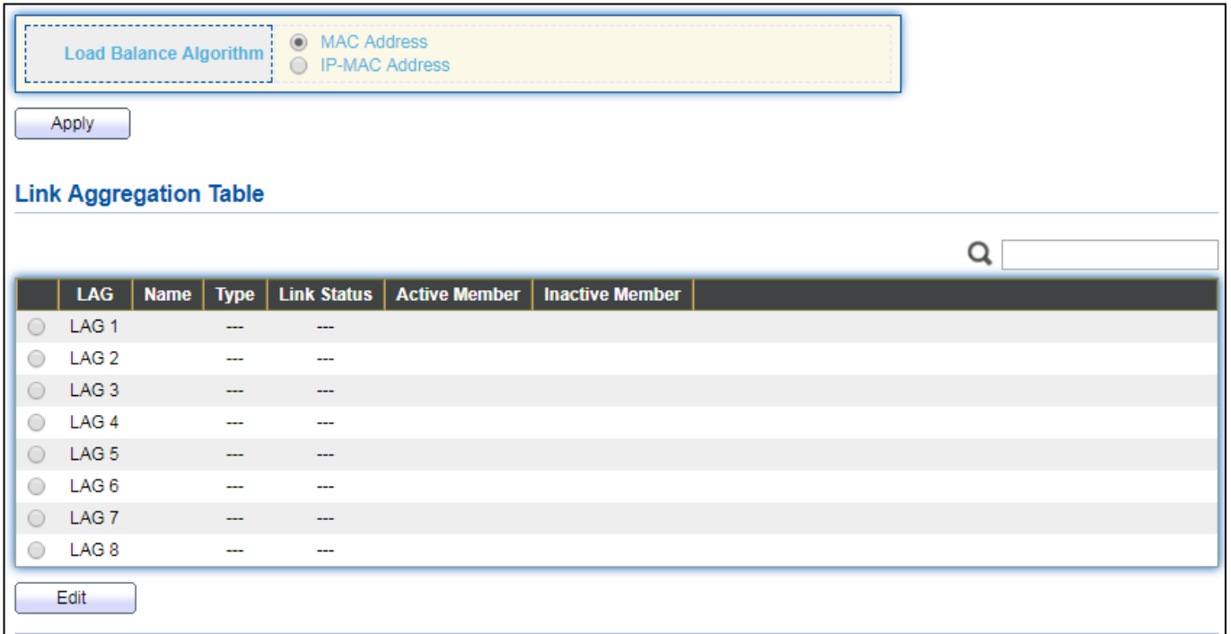
Figure 26 - Port > Link Aggregation > Group
