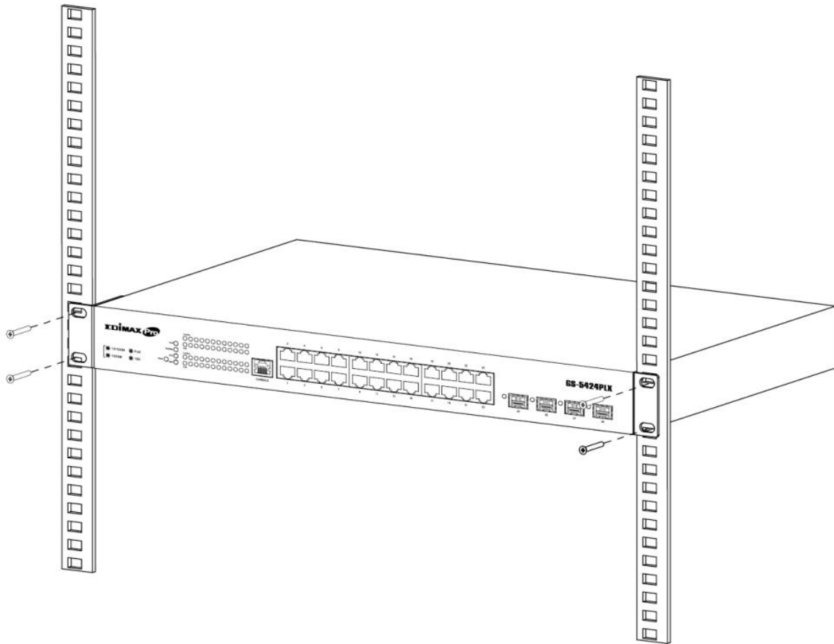
Figure 6 - Rack Installation
