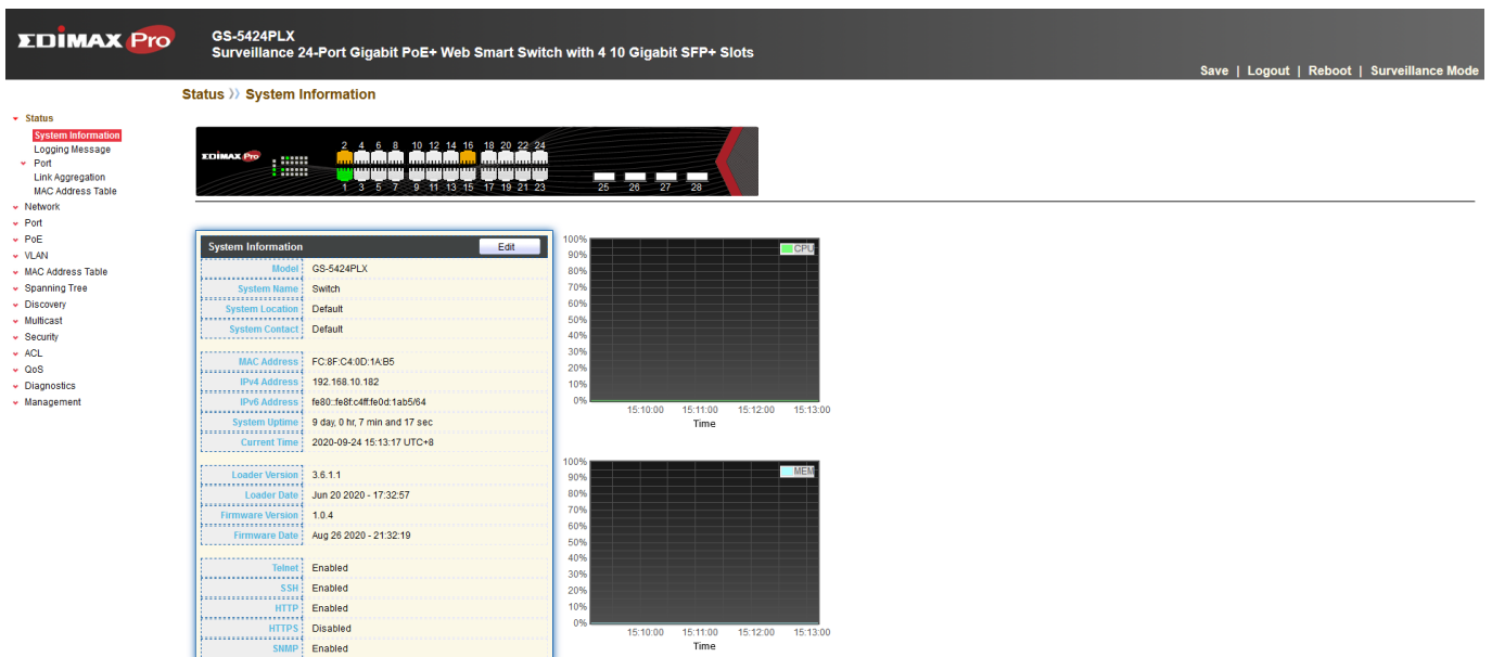
Figure 10 - System Information
