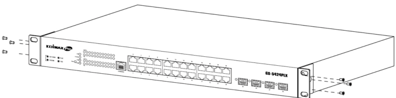
Figure 5 - Bracket Installation
