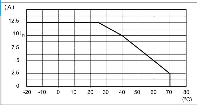
F L78-11 Output current v ambient temperature (78.2E)
