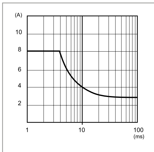
P78-6 Output peak current v time (78.61)
