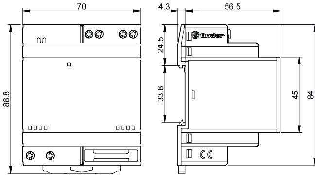
Types 78.51 / 78.61 Screw terminal
