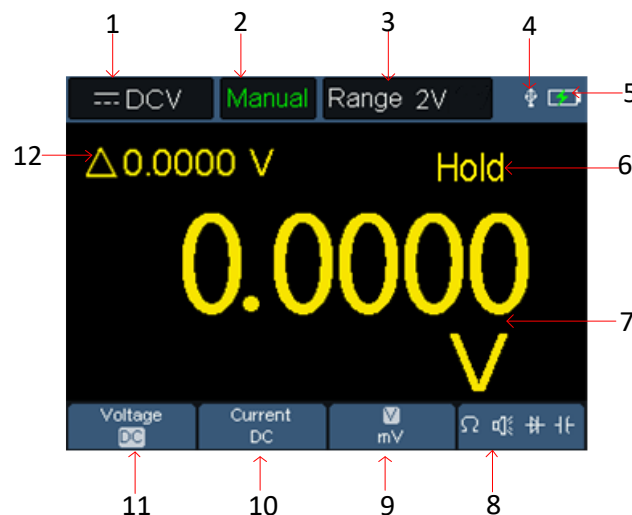
Multimeter Interface
