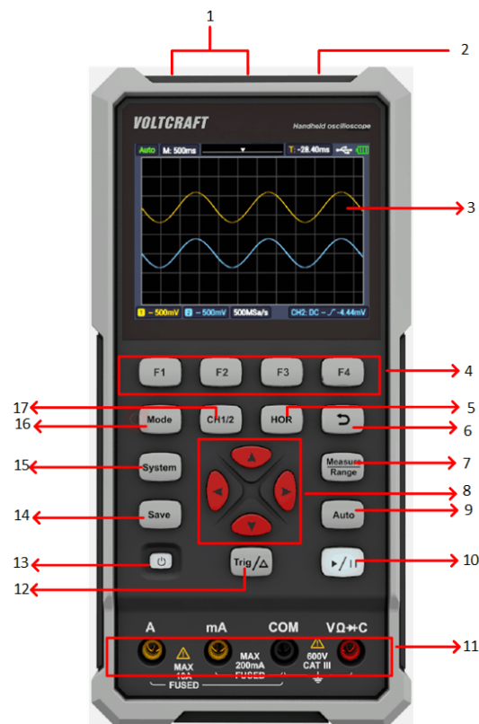
Figure 3-1: Front Panel of the Oscilloscope
