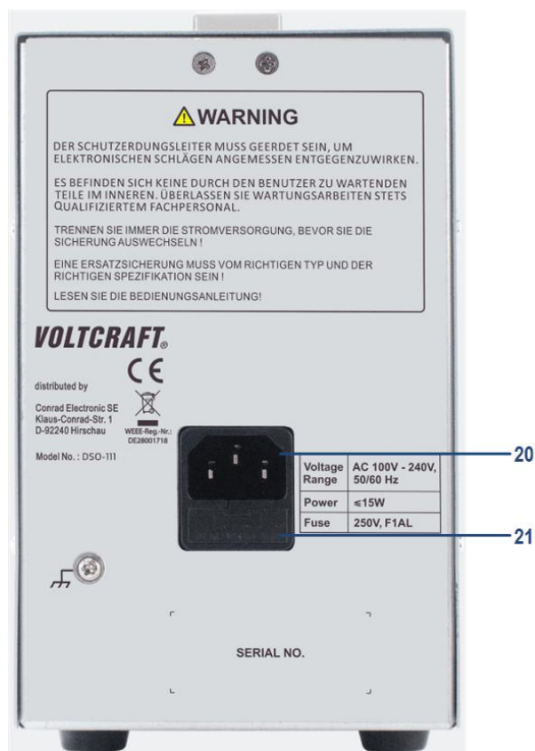
Figure 3-2 Rear Panel
