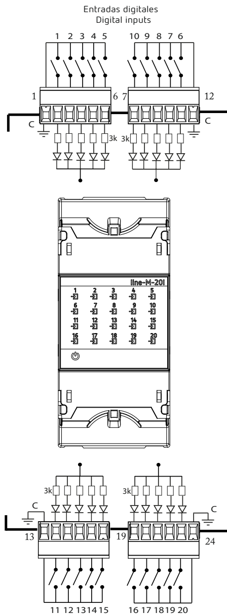
Figure 41: line-M-20I connection diagram.
