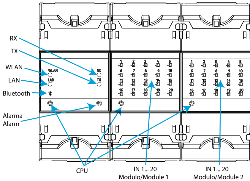
Figure 51: LEDs: line-LM40I-TCP kit.
