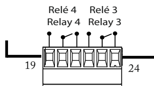
Figure 22: Line-M-4IO-RV connection diagram.
