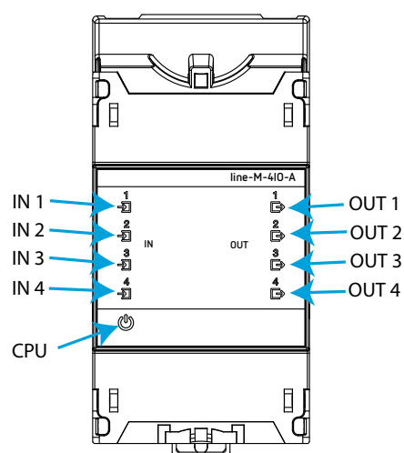
Figure 19: LEDs: line-M-4IO-A.
