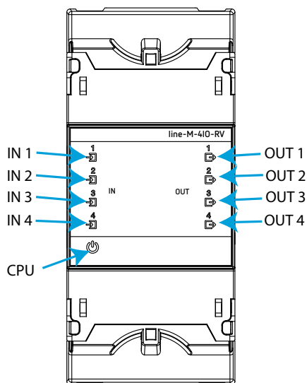
Figure 23: LEDs: line-M-410-RV.
