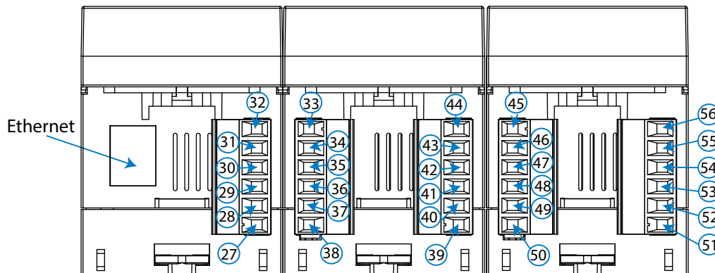
Figure 49: line-LM40I-TCP kit terminals: lower.
