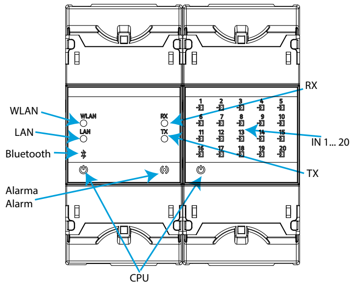
Figure 46: LEDs: line-LM20I-TCP kit.
