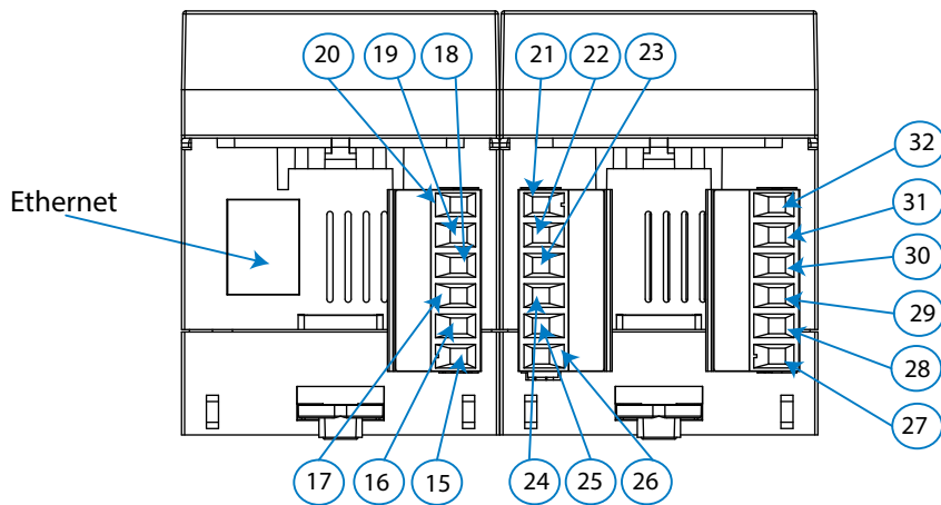
Figure 44: line-LM20I-TCP kit terminals: lower.
