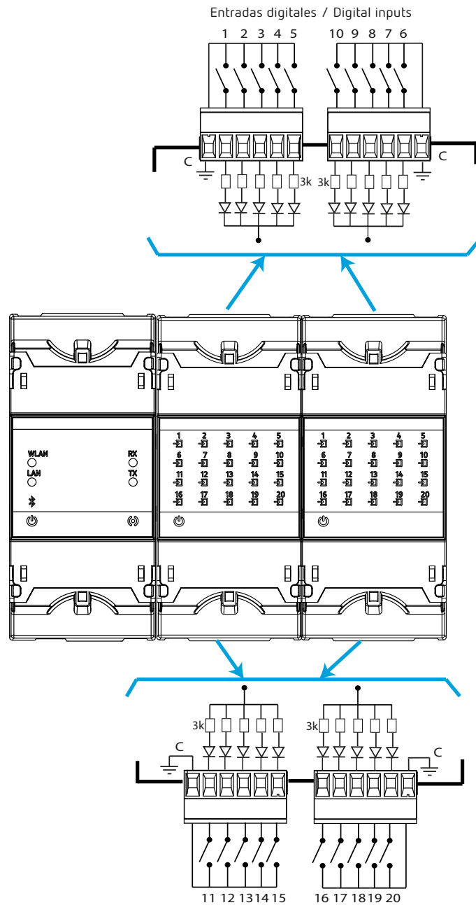
Figure 50: line-LM40I-TCP kit connection diagram.
