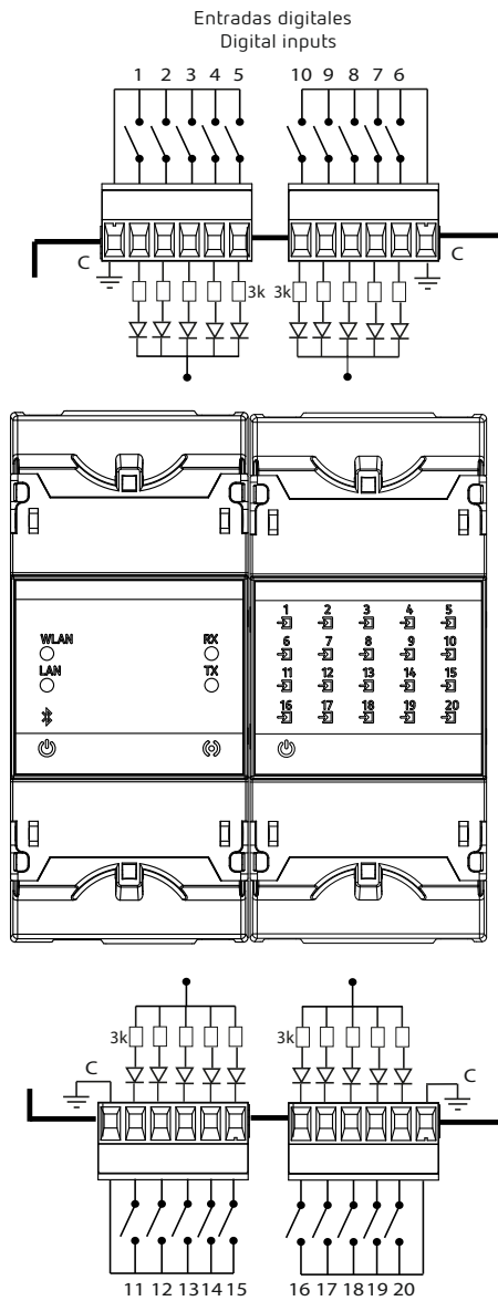
Figure 45: line-LM201-TCP kit connection diagram.
