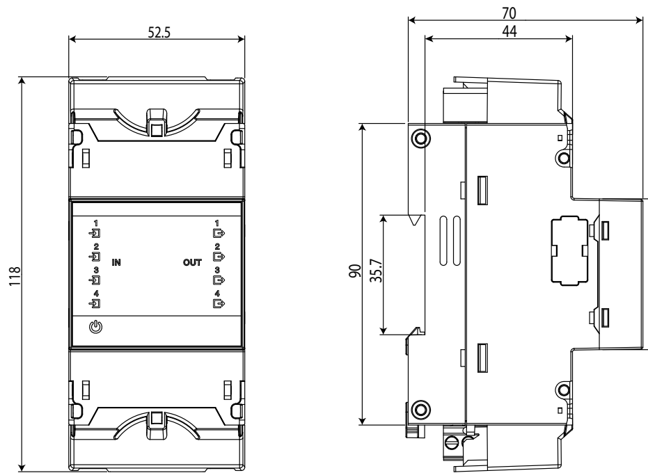
Figure 12: Line-M dimensions.
