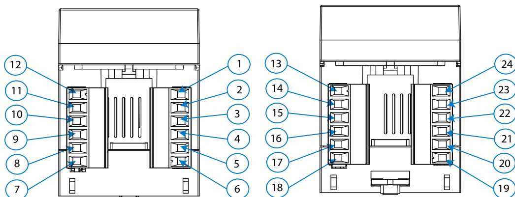
Figure 40: line-M-20I terminals: Upper - lower.
