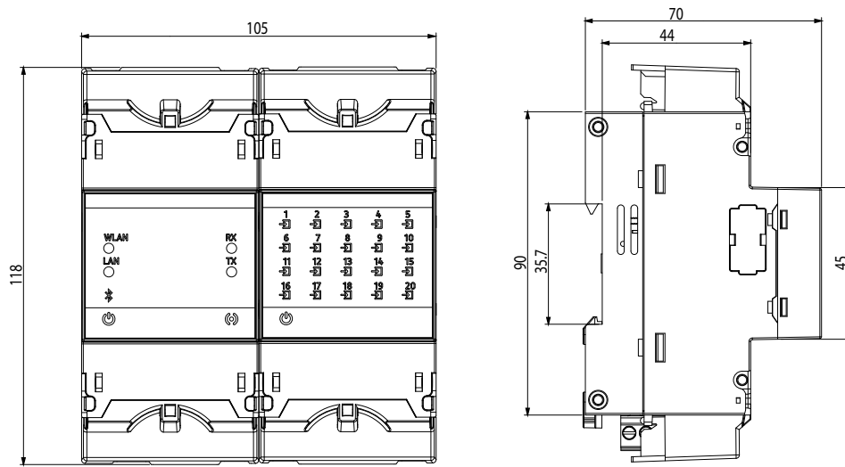
Figure 47: line-LM20I-TCP kit dimensions.
