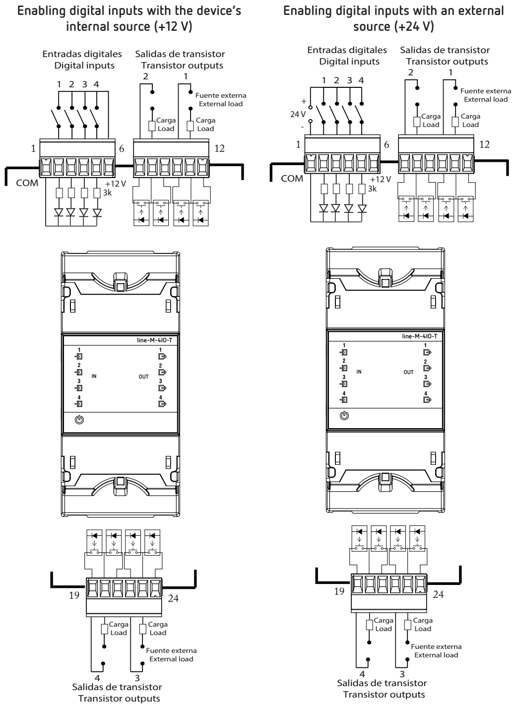
Figure 14: Line-M-410-T connection diagram.
