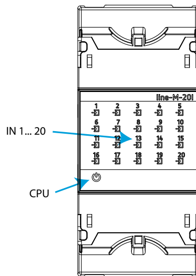
Figure 42: LEDs: line-M-20I.
