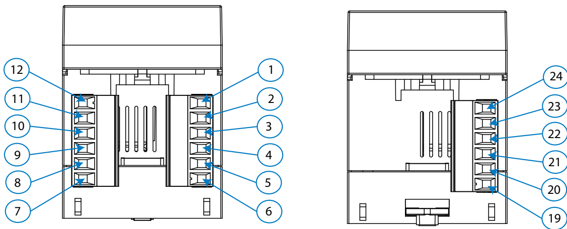
Figure 13: Line-M-410-T terminals: Upper - Lower.
