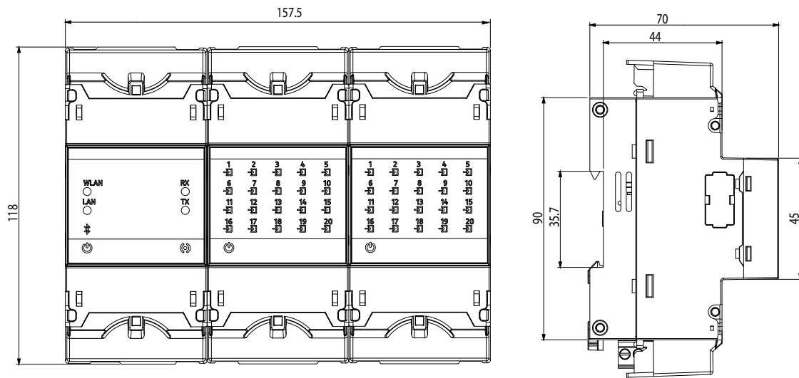
Figure 52: line-LM40I-TCP kit dimensions.
