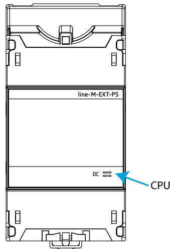
Figure 30: LEDs: line-M-EXT-PS.
