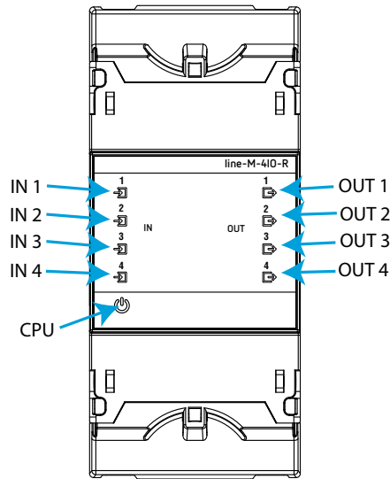
Figure 10: LEDs: line-M-4IO-R.
