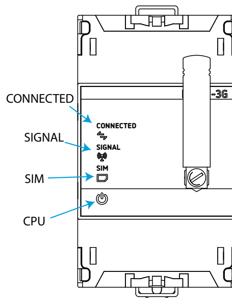
Figure 32: LEDs: line-M-3G.
